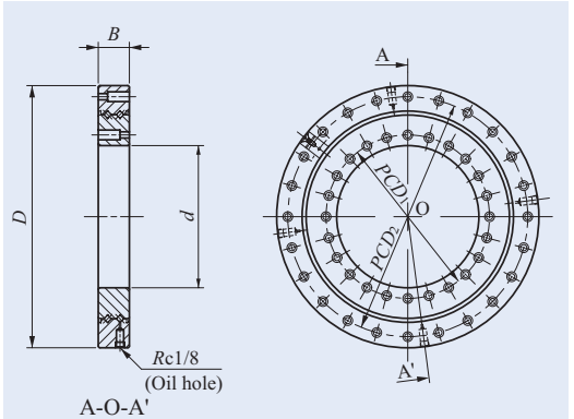
Fig. 7 Manufacturing example
