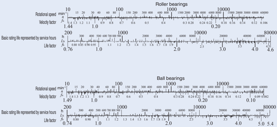
Fig. 2 Scales for rating life calculation
