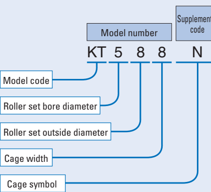
(b) Example of "Bore diameter or roller set bore diameter + Outside diameter or roller set outside diameter + width"
